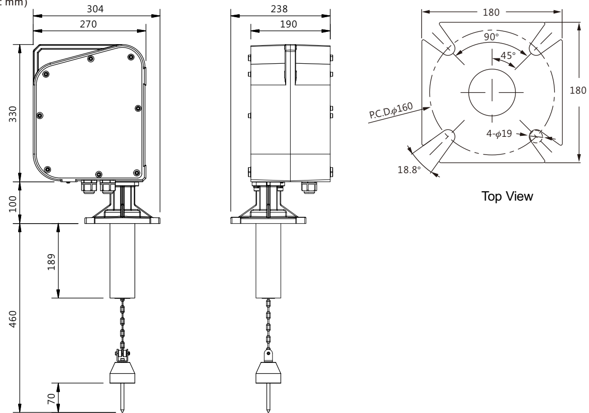
Front View
